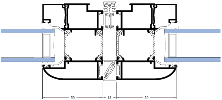
SOFT LINE CROWN SLIDING FOLDING DOOR
