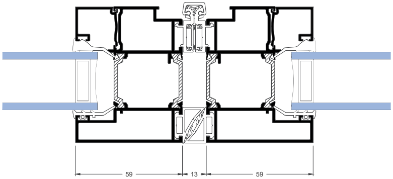
SLIM LINE CROWN SLIDING FOLDING DOOR
