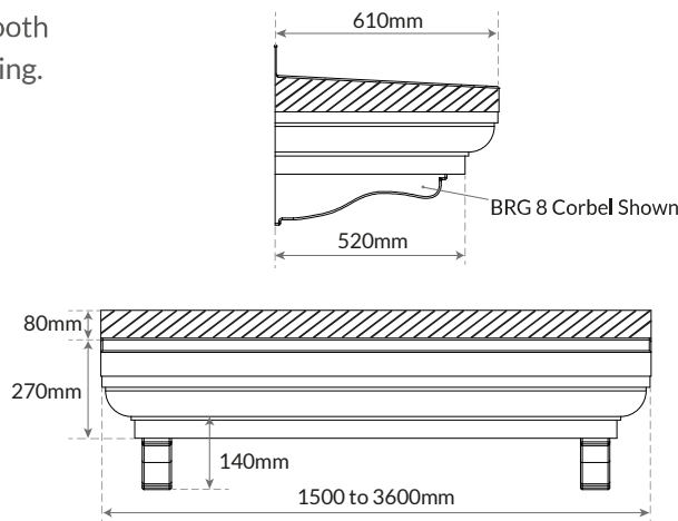
Lead effect top with GRP corbels (BRG8)
