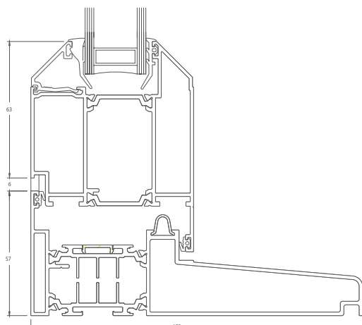
Integrated cill option
