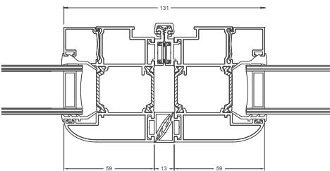
Softline Crown Sliding Folding Door
