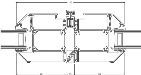
Original Crown Sliding Folding Door
