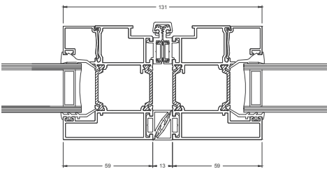
Slimline Crown Sliding Folding Door
